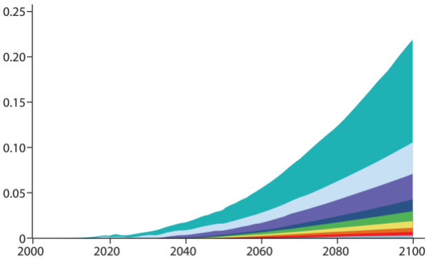
Global sea level contribution, m
