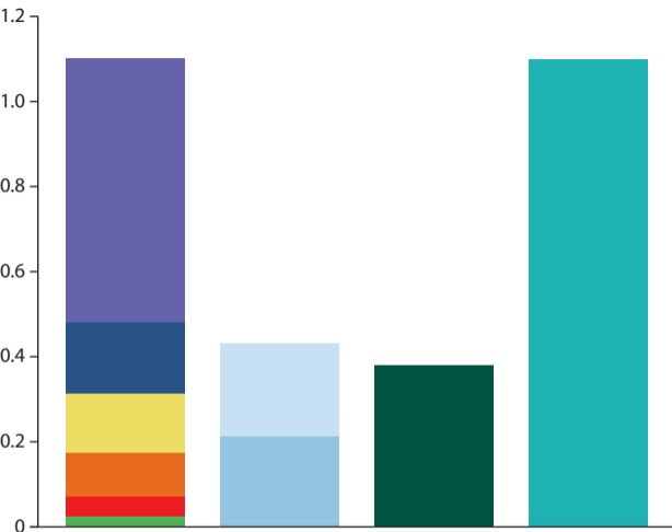
Sea level contribution, mm/y
