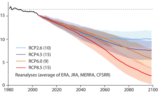
Permafrost area, million km 2
