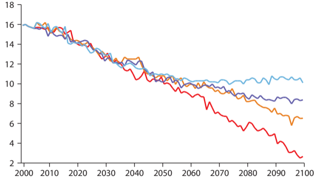
Permafrost area, million km 2
