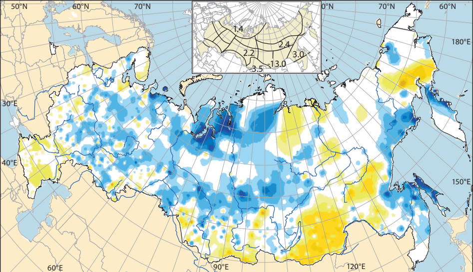
SDmax trend, cm/decade
