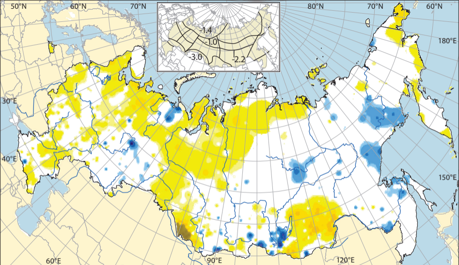
Snow cover trend, days/decade
