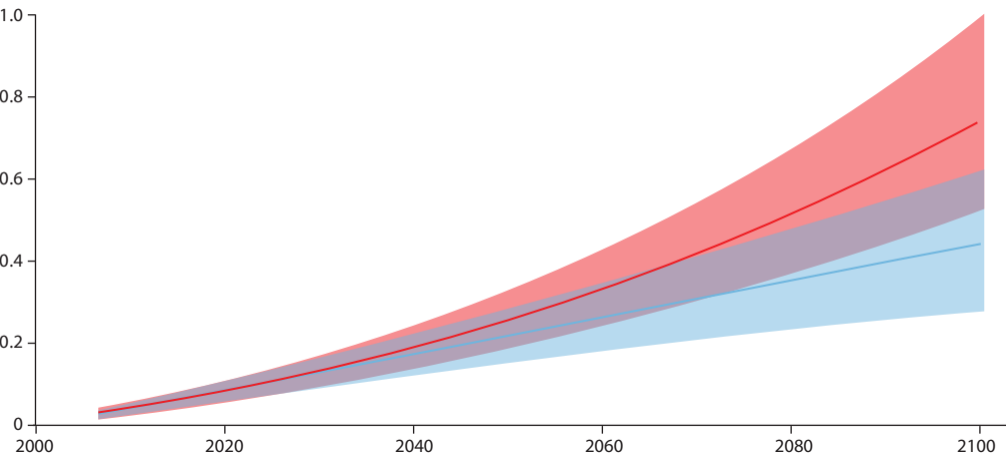
Global mean sea-level rise, m
