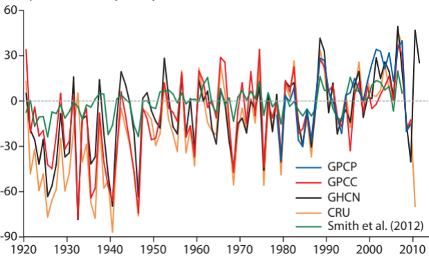
Precipitation anomaly, mm/y
