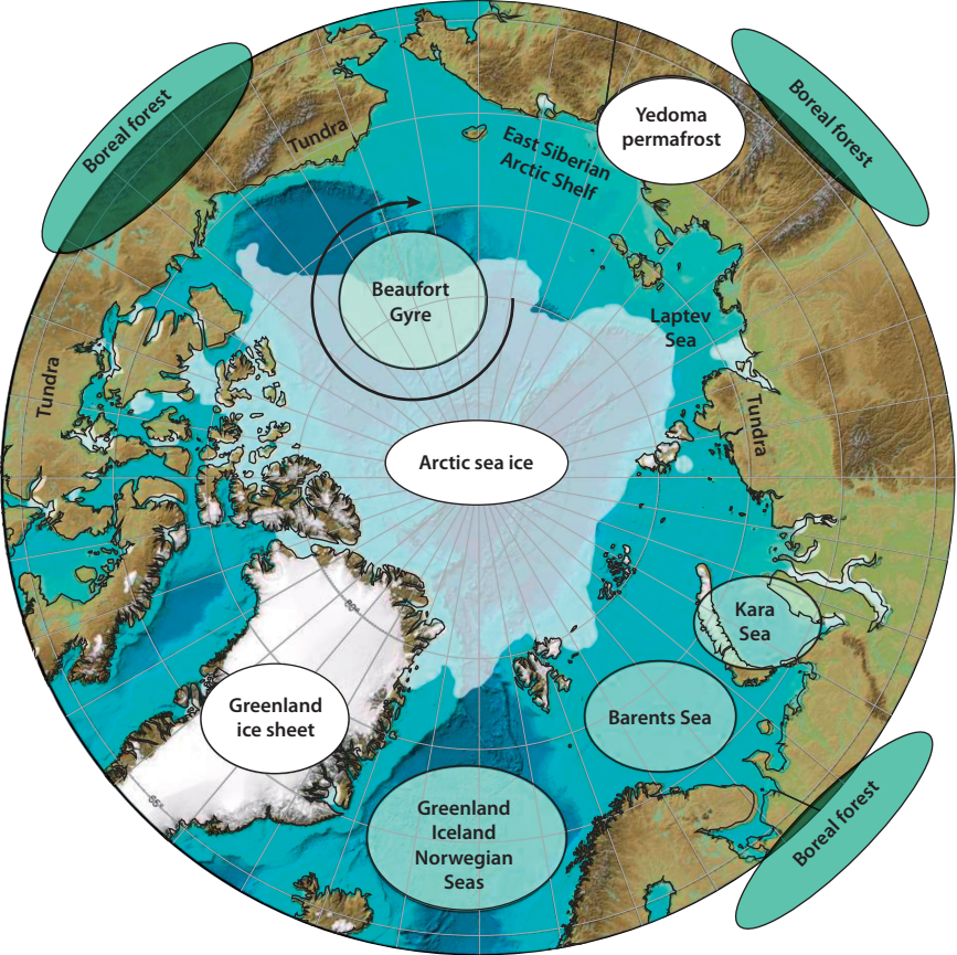
Bathymetry and topography, m
