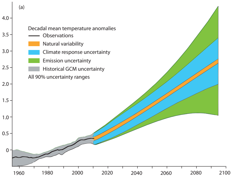
Change in global average temperature, °C
