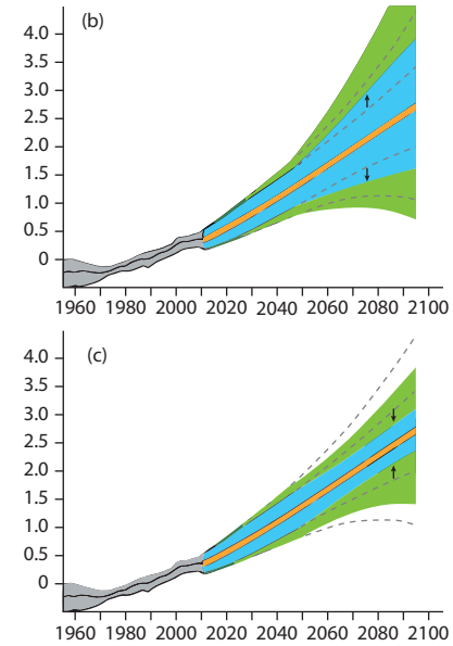
Change in global average temperature, °C
