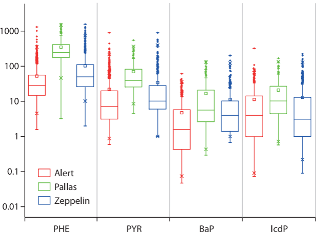
Concentration ranges of PAHs, \text{pg}/\text{m}^3
