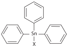
Triphenyl tin (TPT)
