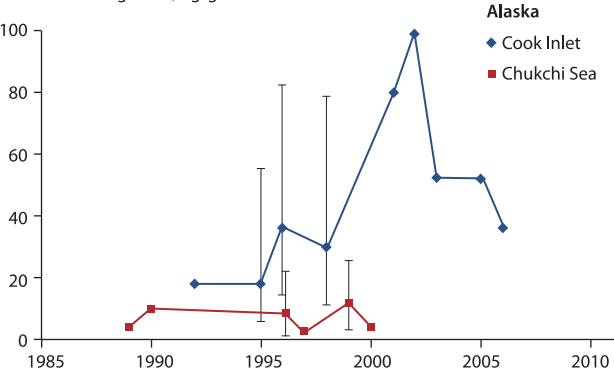
\Sigma PFCAs in beluga liver, ng/g ww
