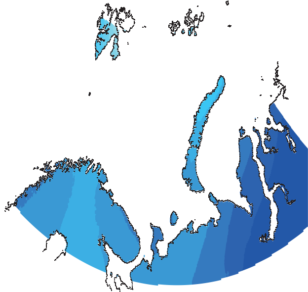
Change in precipitation, %
