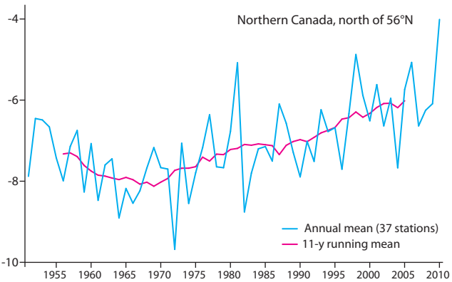
Annual mean air temperature, °C
