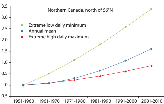
Change in air temperature, °C
