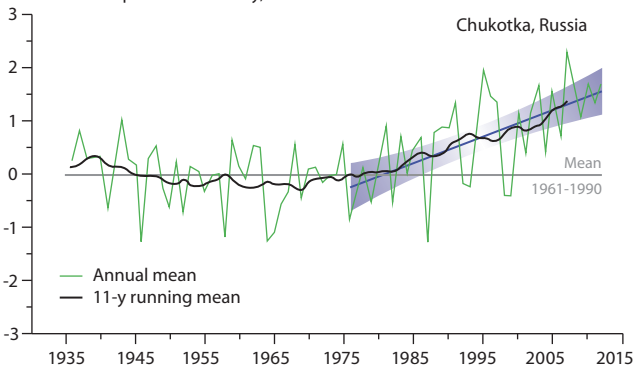
Surface air temperature anomaly, °C
