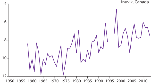
Annual mean air temperature, °C
